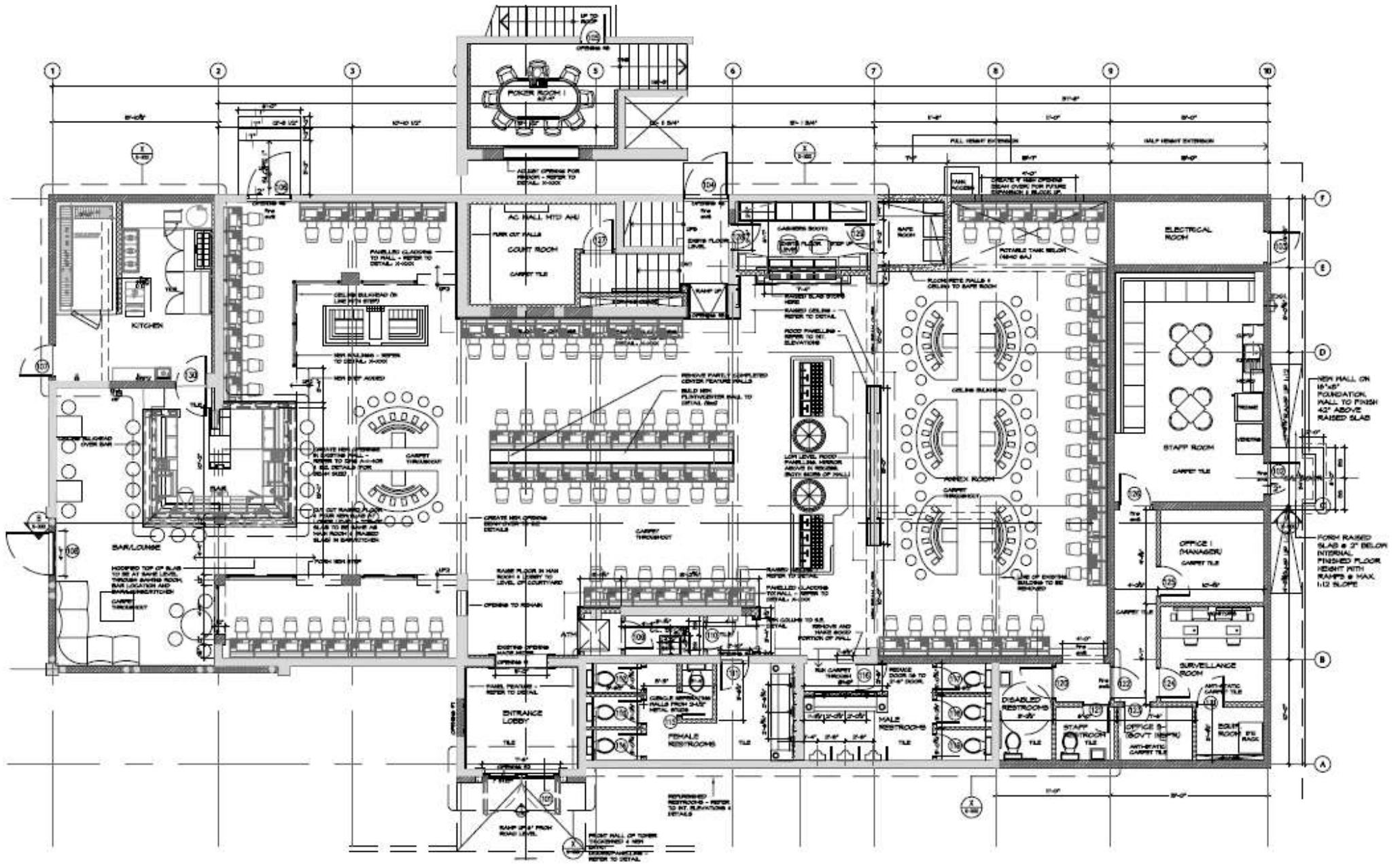
LEVEL 1 PLAN - Scale: 1"=10'
