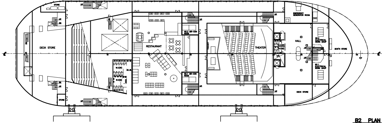
B2 PLAN
