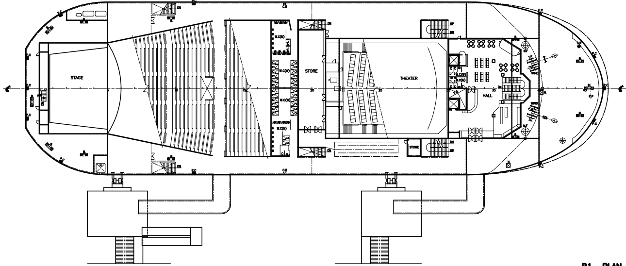
B1 PLAN
